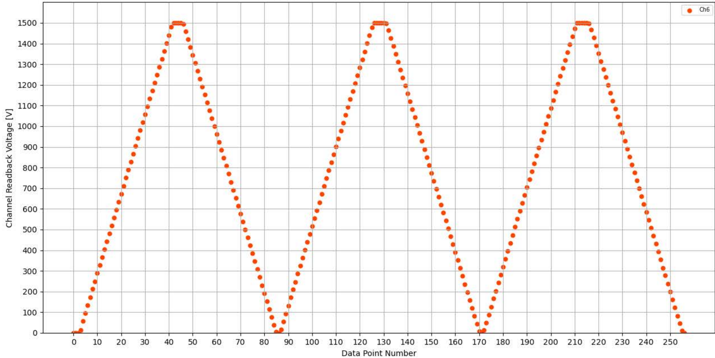
Voltage Ramp Test (Python) Bd #359, Slot #3, Ch #6
