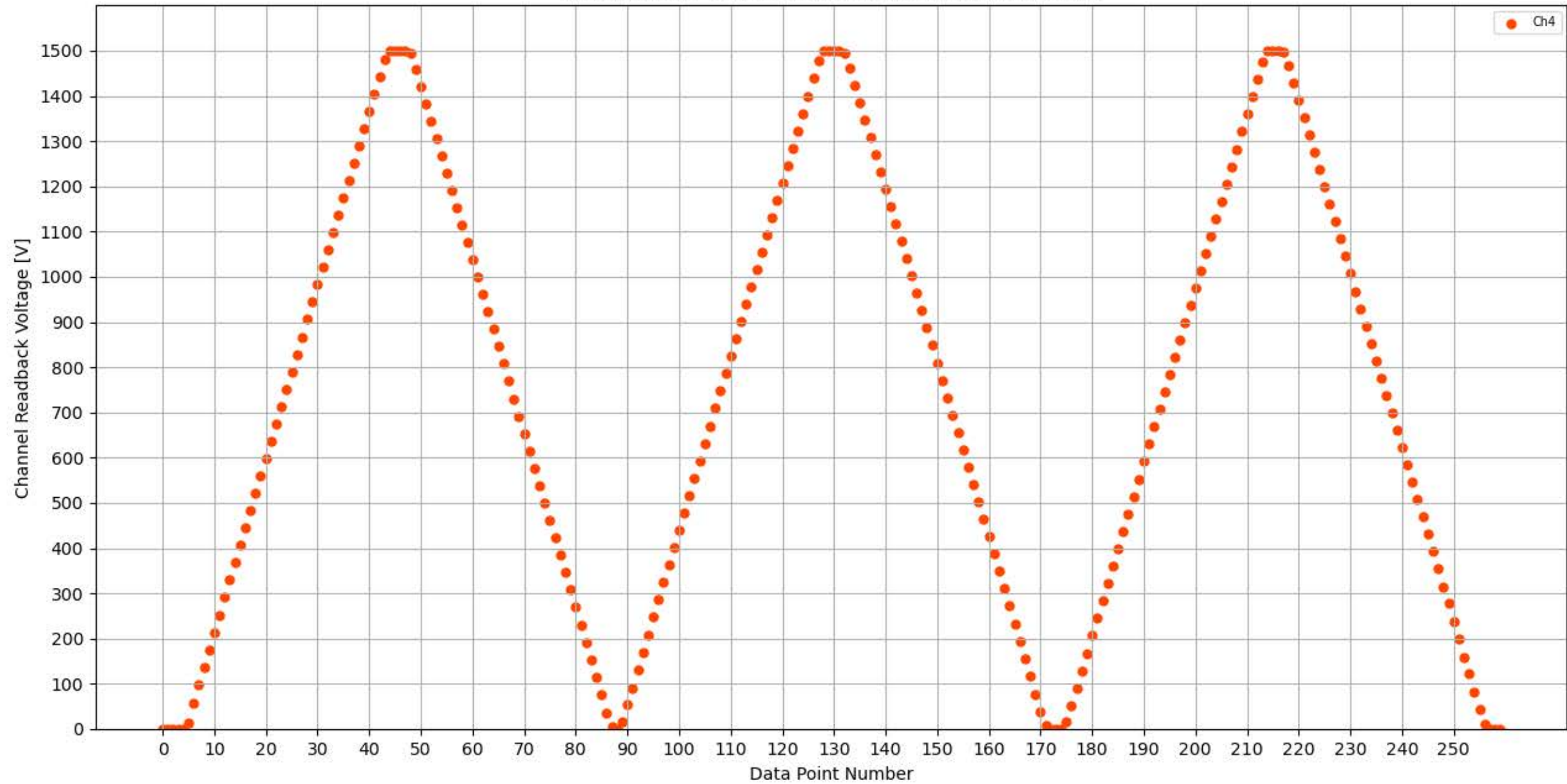
Voltage Ramp Test (Python) Bd #359, Slot #3, Ch #4
