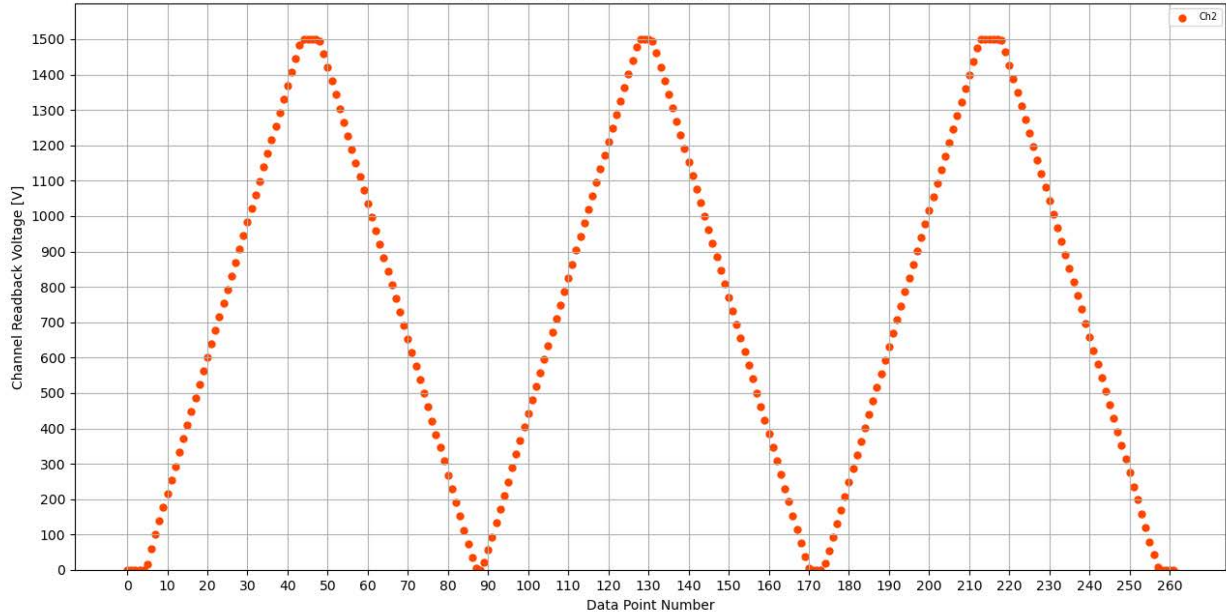
Voltage Ramp Test (Python) Bd #359, Slot #3, Ch #2
