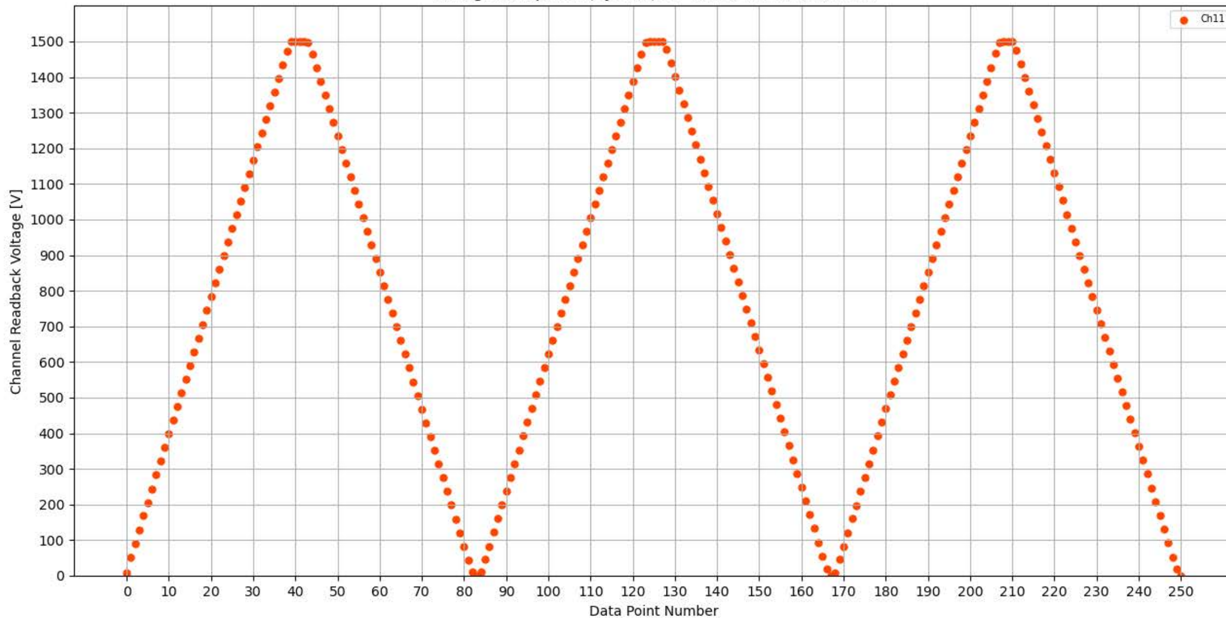
Voltage Ramp Test (Python) Bd #359, Slot #3, Ch #11
