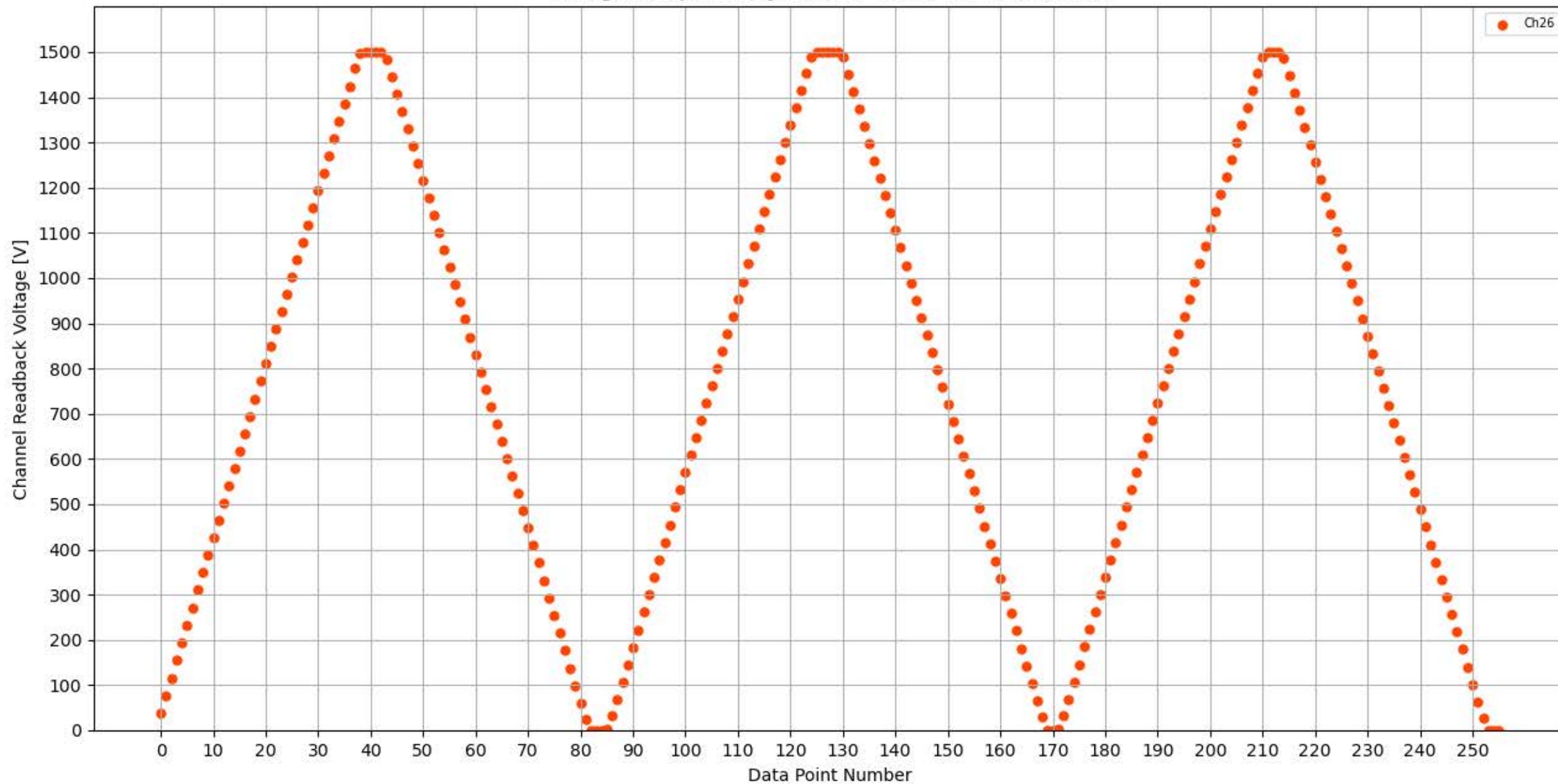
Voltage Ramp Test (Python) Bd #359, Slot #3, Ch #26
