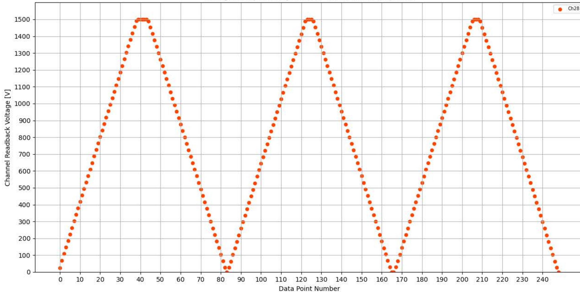
Voltage Ramp Test (Python) Bd #359, Slot #3, Ch #28
