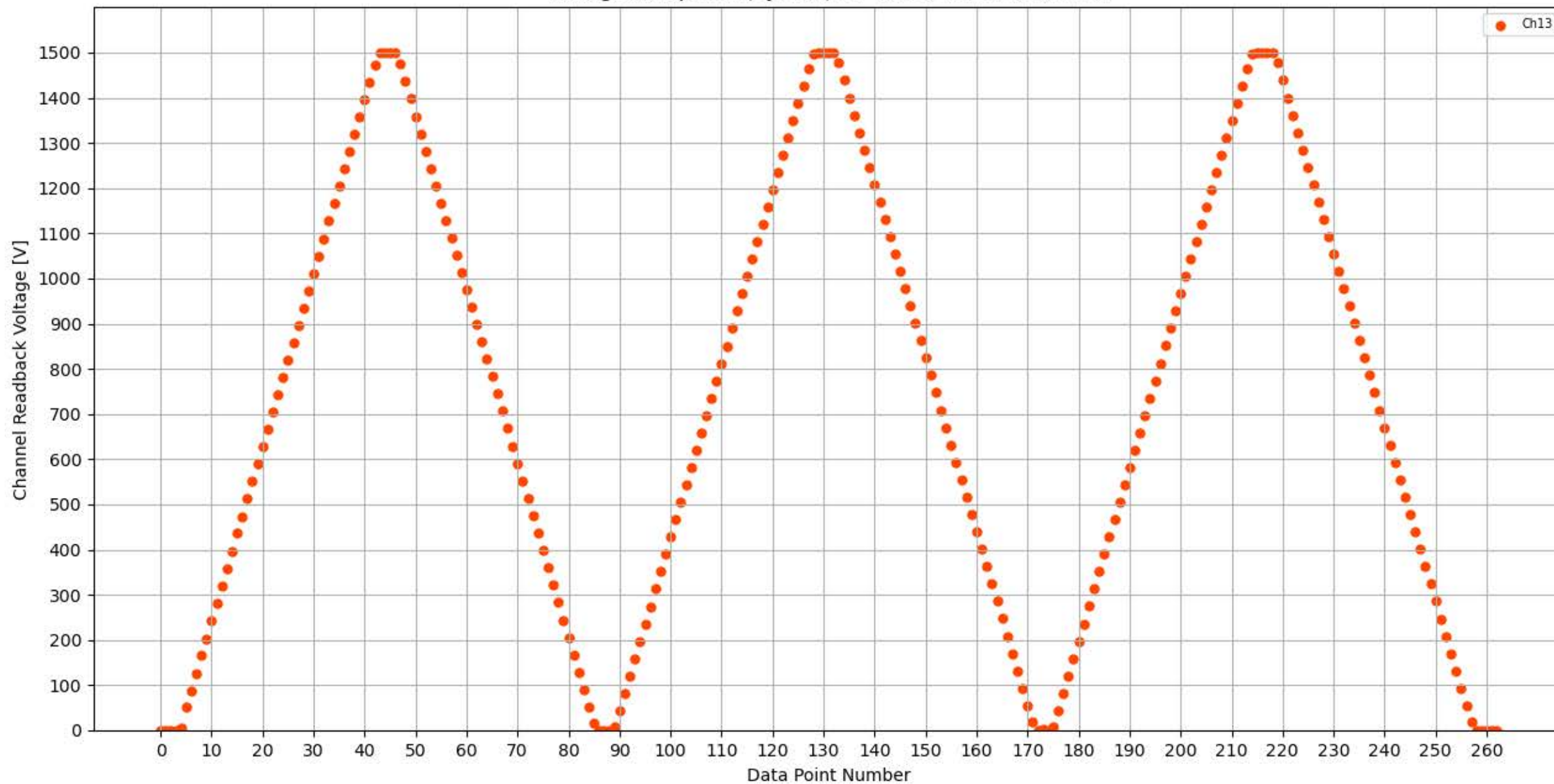
Voltage Ramp Test (Python) Bd #359, Slot #3, Ch #13
