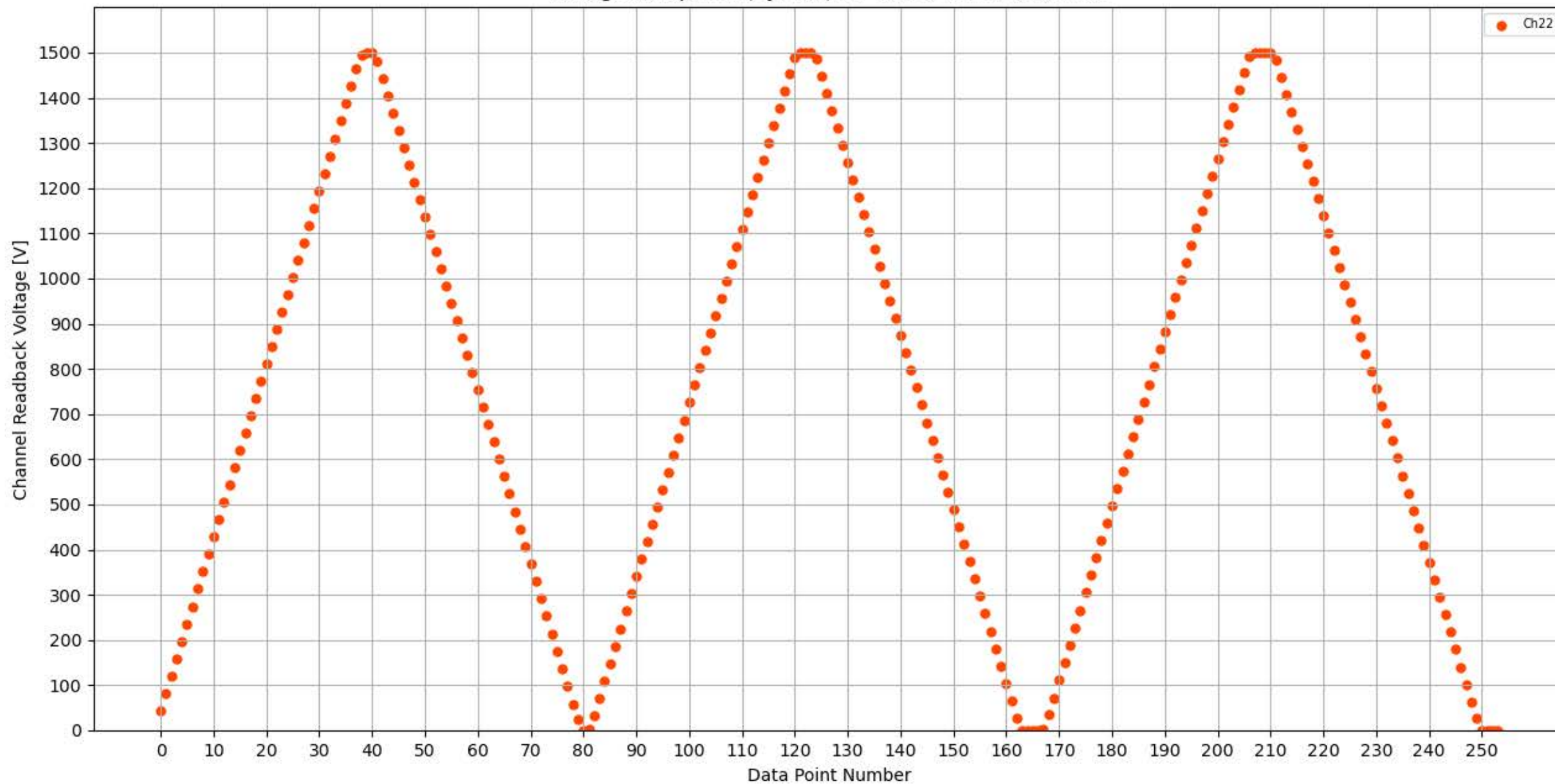
Voltage Ramp Test (Python) Bd #359, Slot #3, Ch #22
