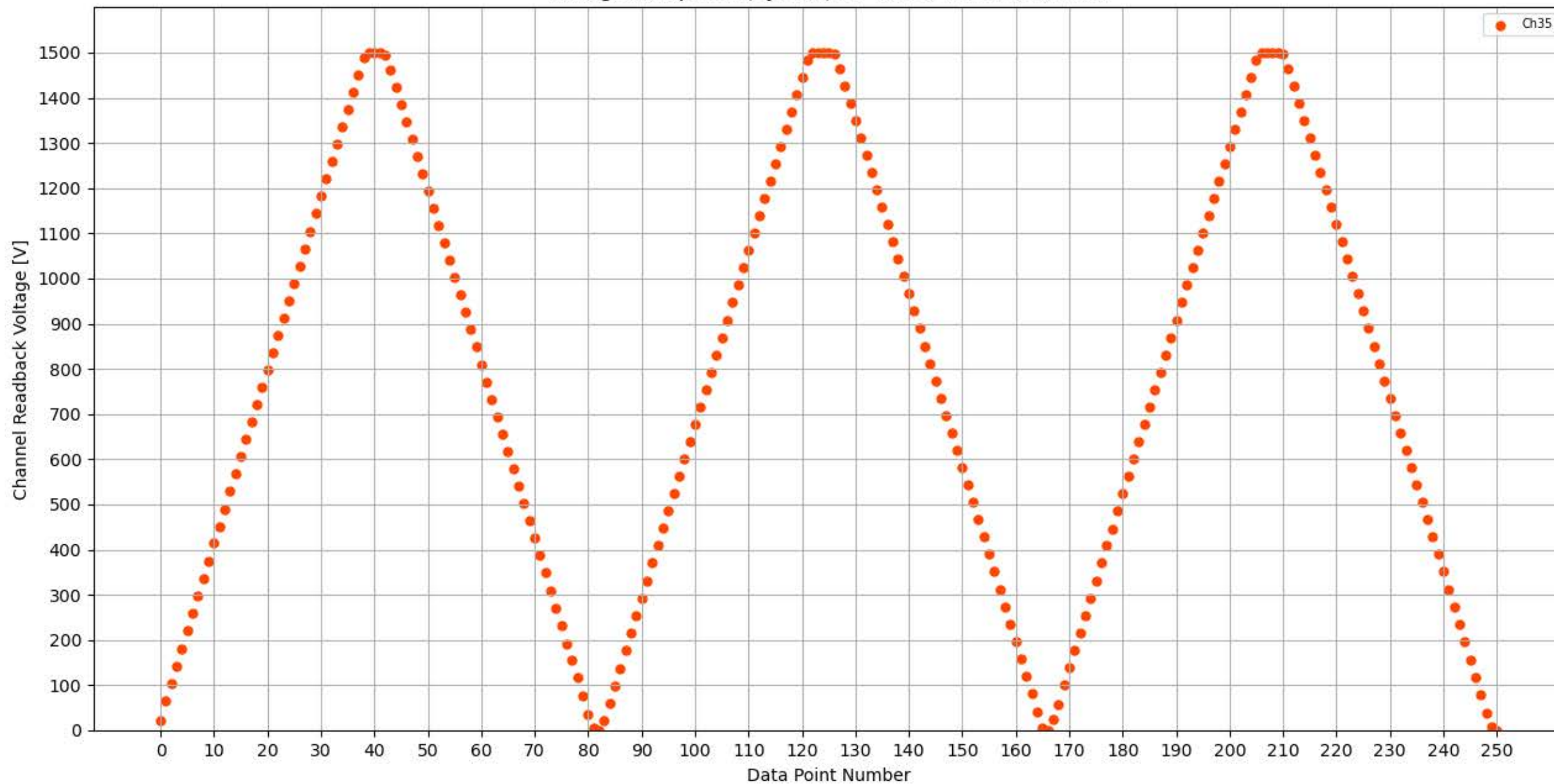
Voltage Ramp Test (Python) Bd #359, Slot #3, Ch #35
