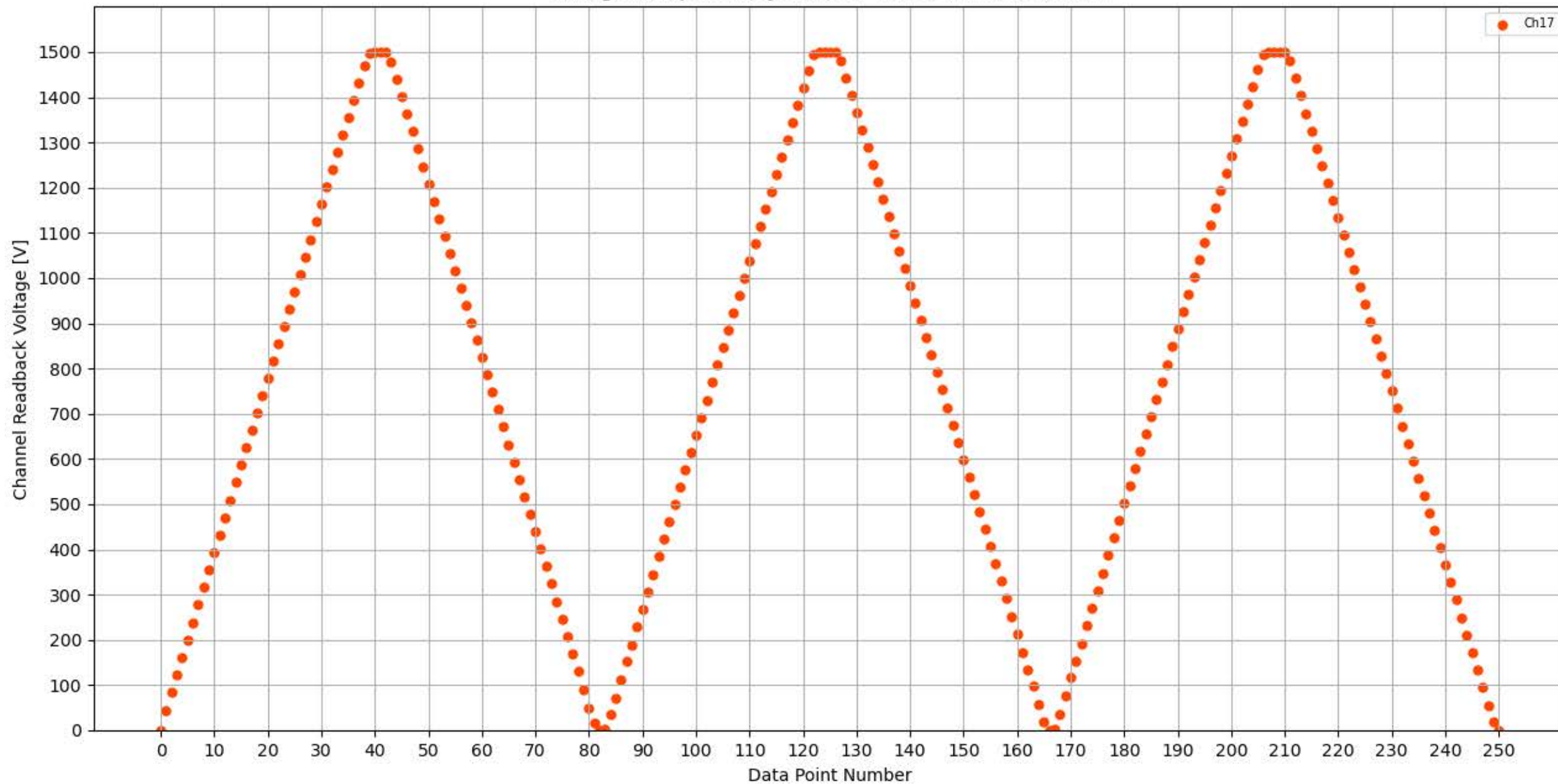
Voltage Ramp Test (Python) Bd #359, Slot #3, Ch #17
