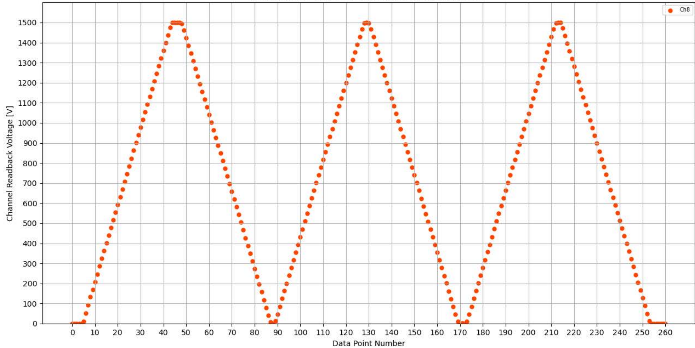
Voltage Ramp Test (Python) Bd #359, Slot #3, Ch #8
