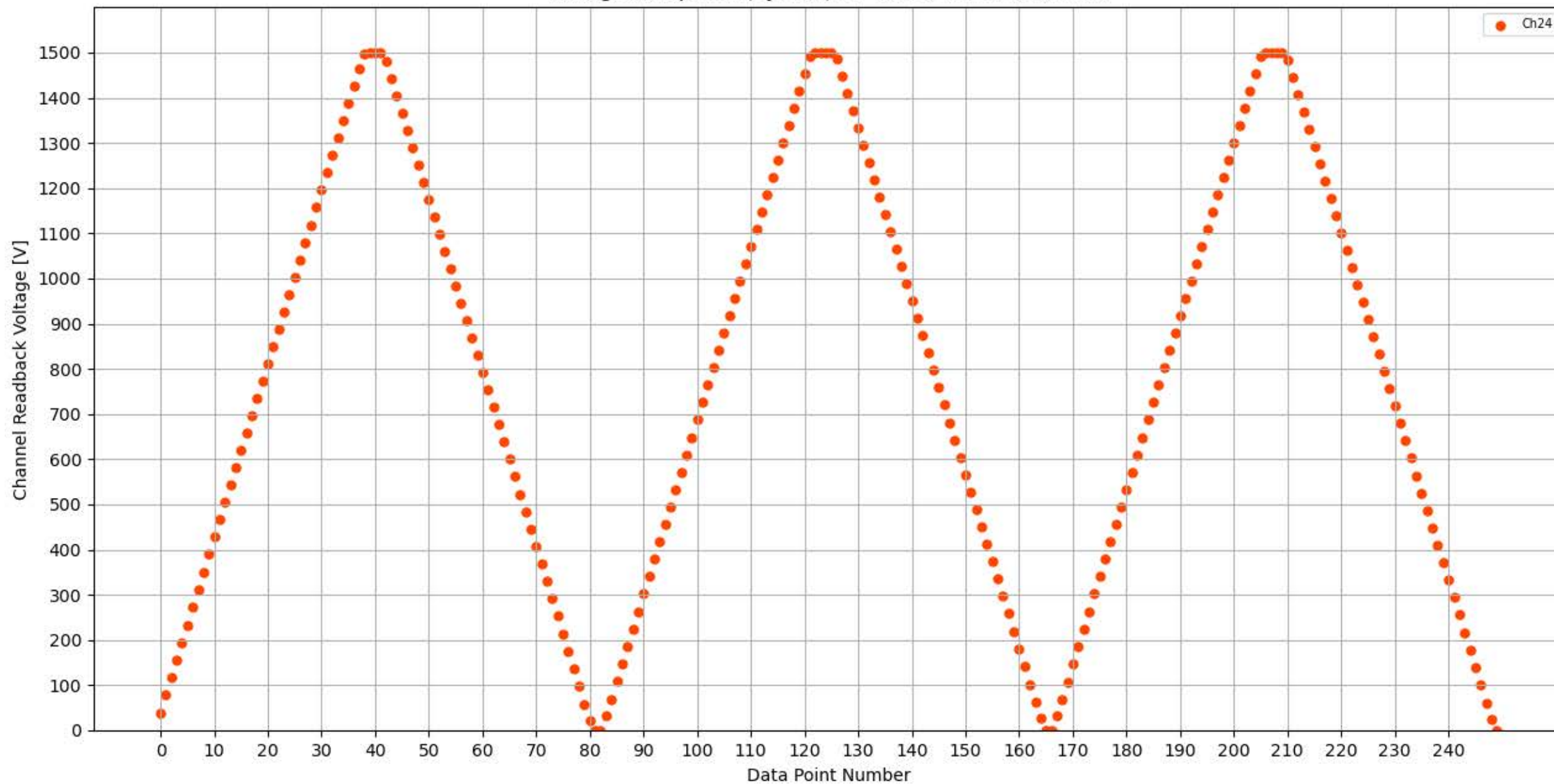
Voltage Ramp Test (Python) Bd #359, Slot #3, Ch #24
