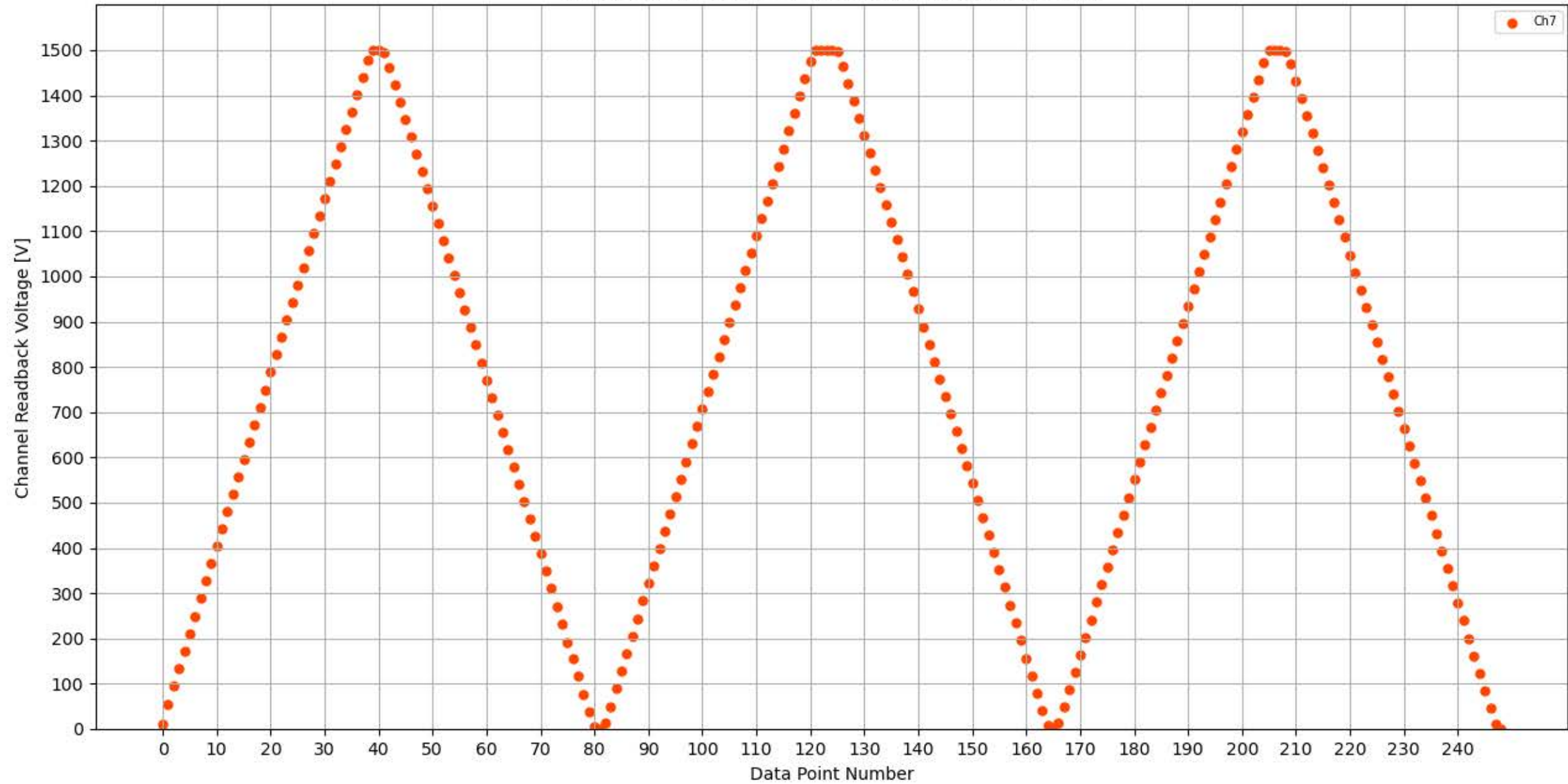
Voltage Ramp Test (Python) Bd #359, Slot #3, Ch #7
