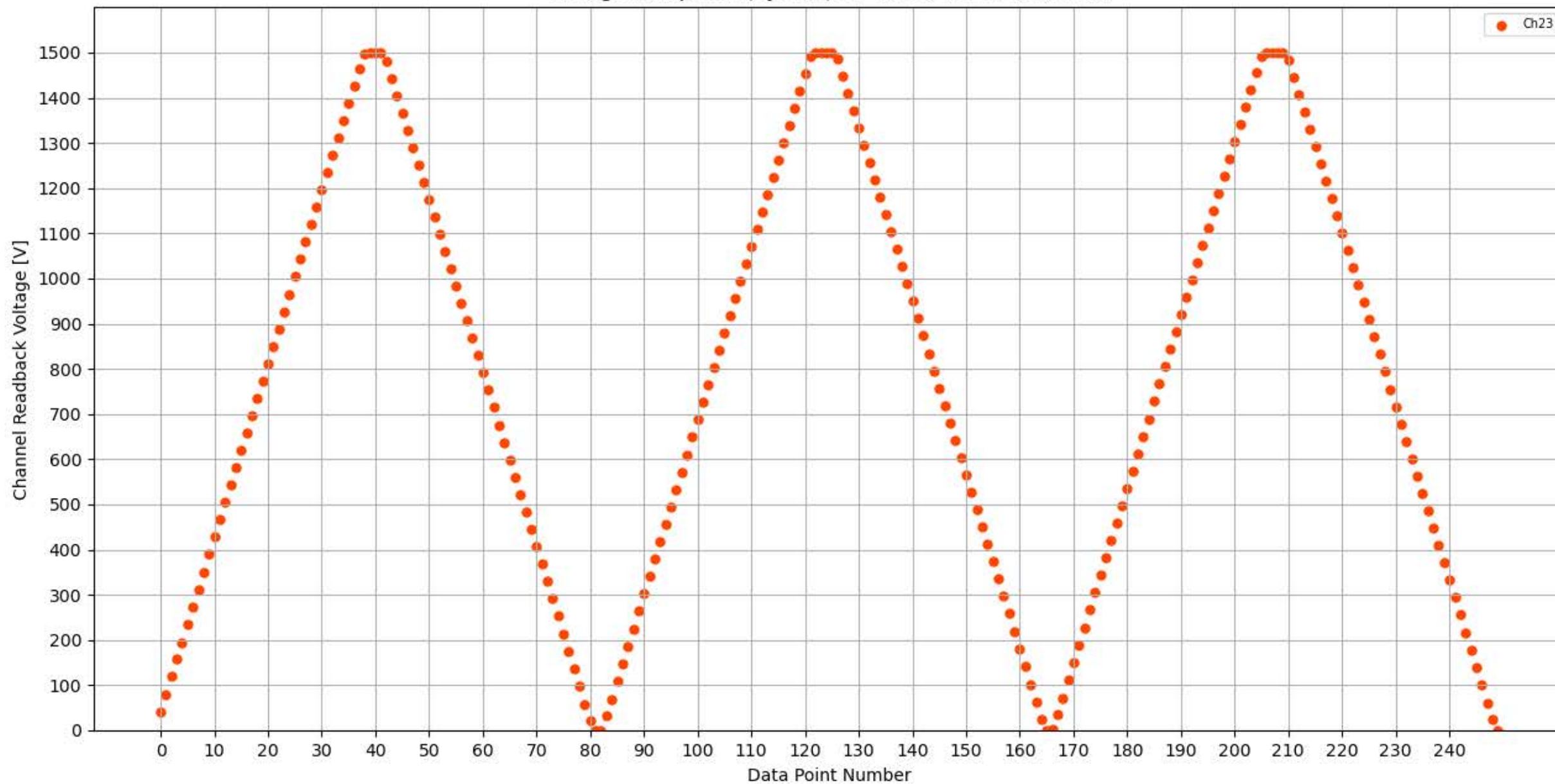
Voltage Ramp Test (Python) Bd #359, Slot #3, Ch #23
