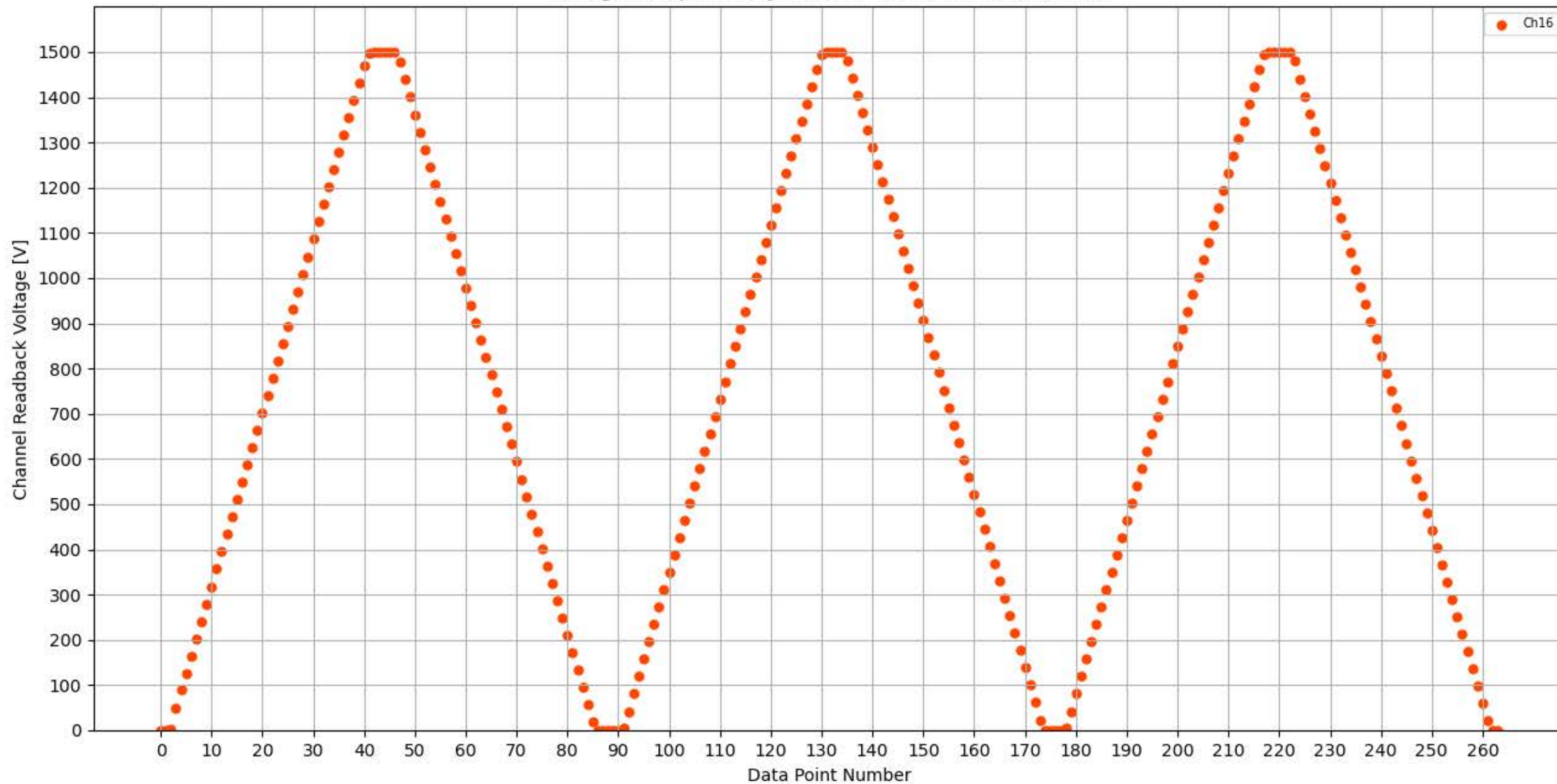
Voltage Ramp Test (Python) Bd #359, Slot #3, Ch #16
