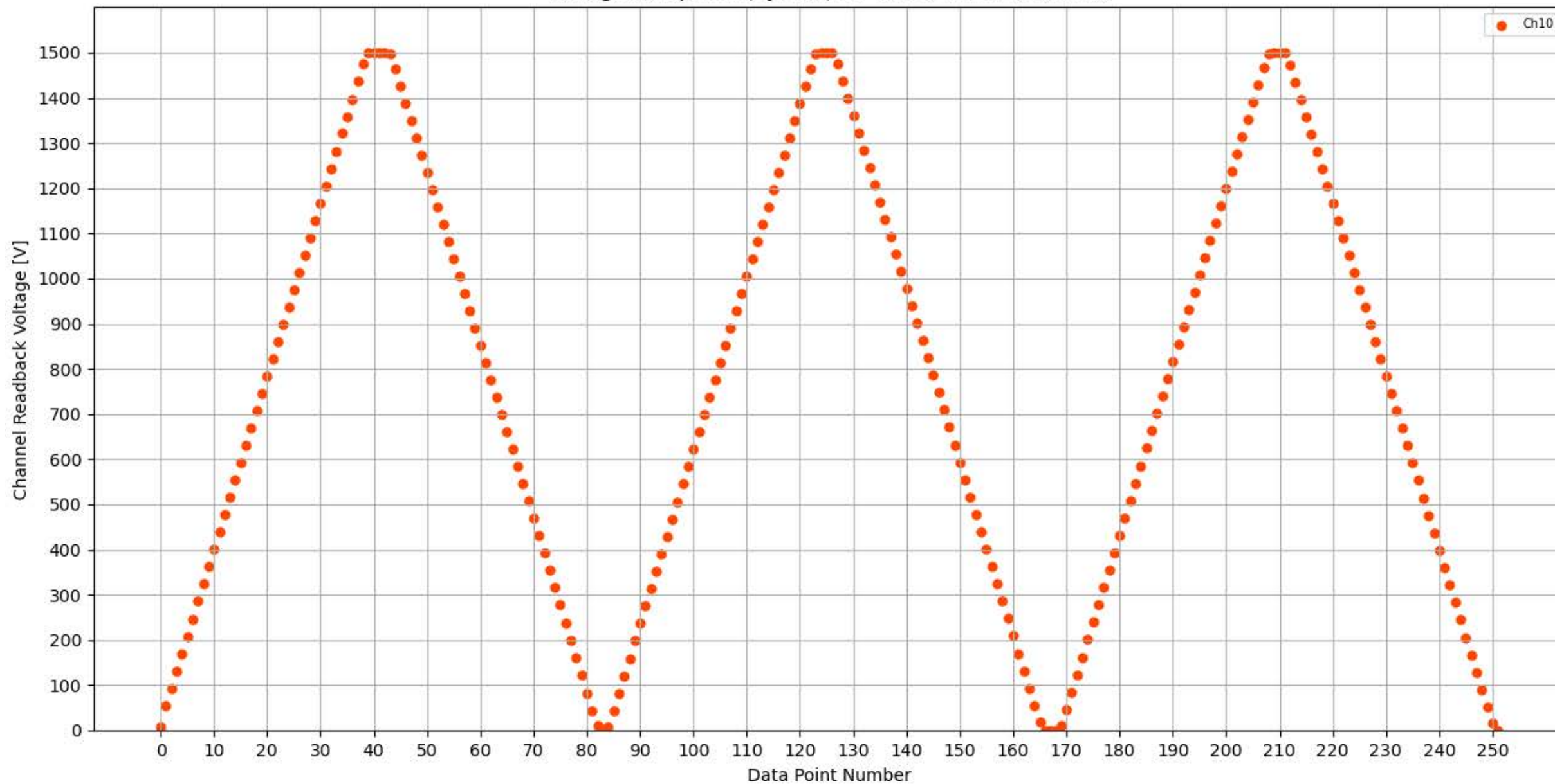
Voltage Ramp Test (Python) Bd #359, Slot #3, Ch #10
