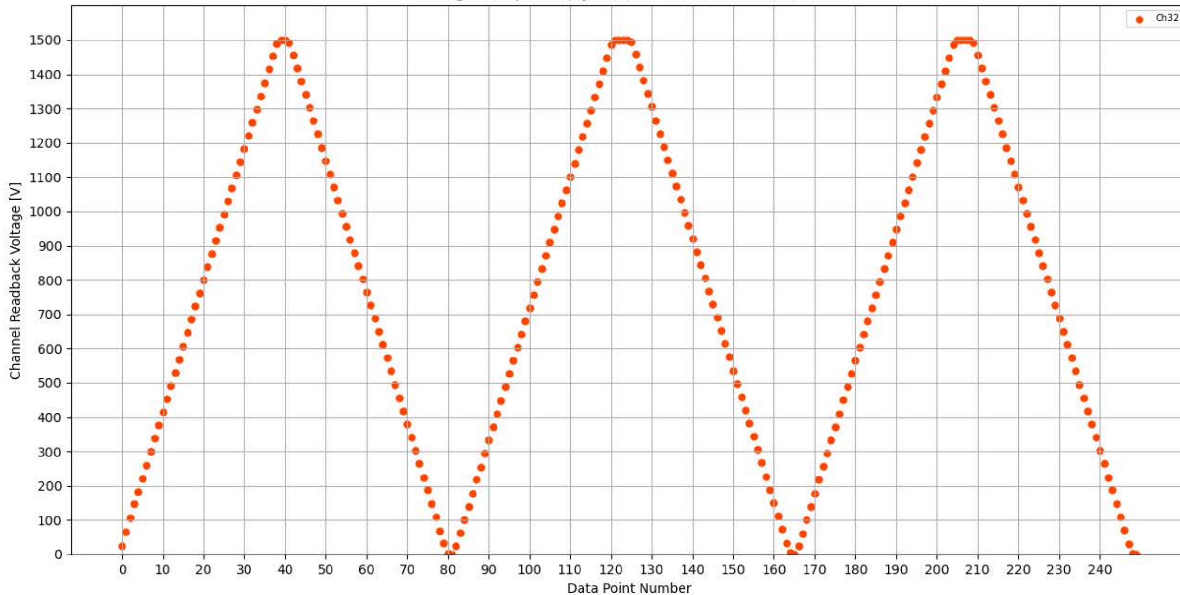
Voltage Ramp Test (Python) Bd #359, Slot #3, Ch #32
