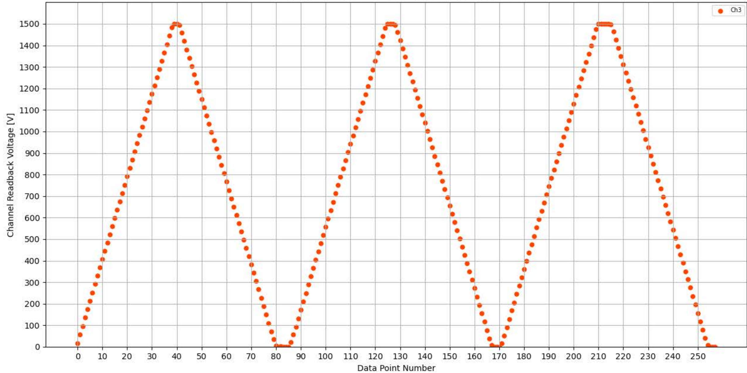
Voltage Ramp Test (Python) Bd #359, Slot #3, Ch #3
