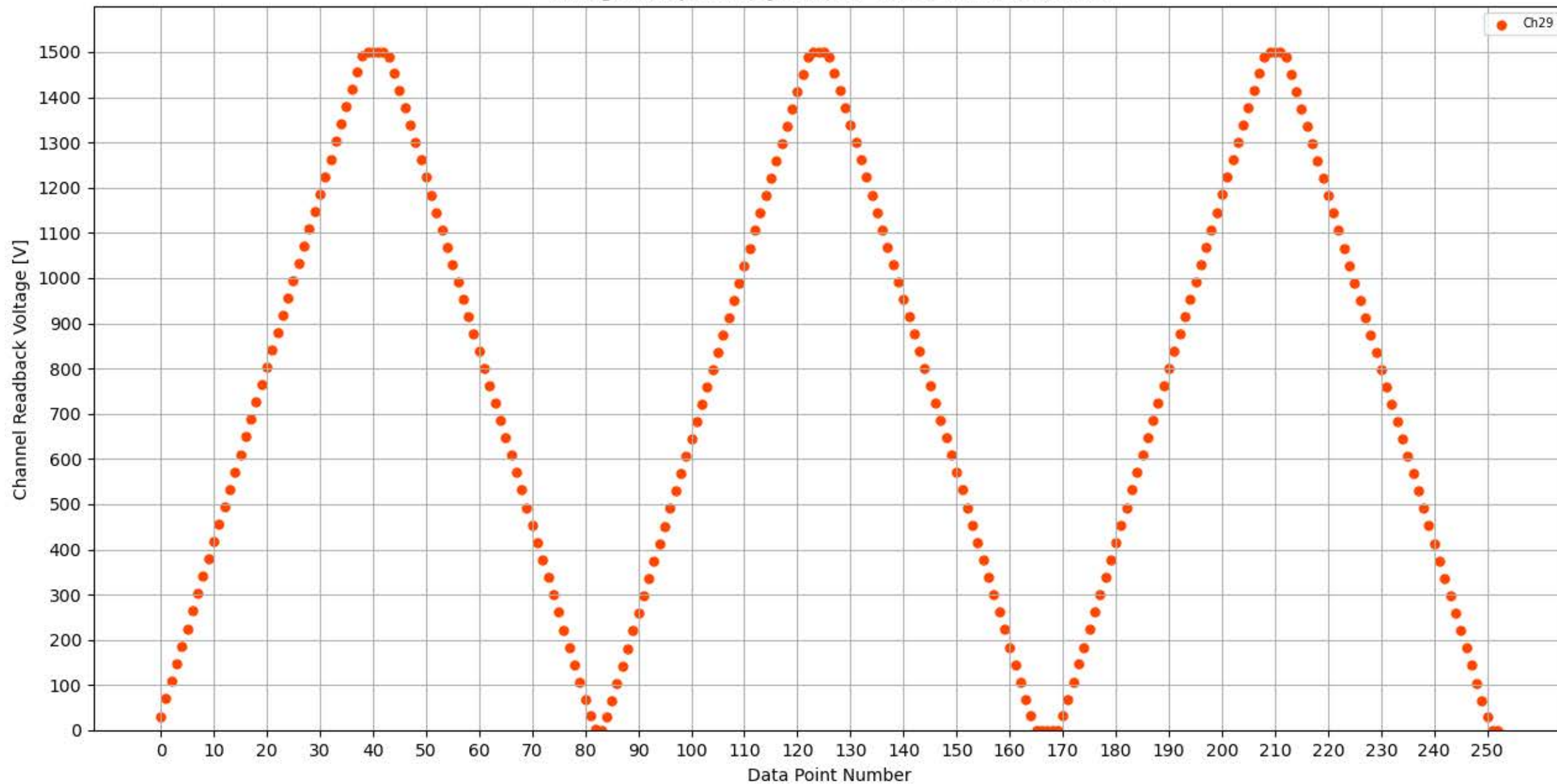
Voltage Ramp Test (Python) Bd #359, Slot #3, Ch #29
