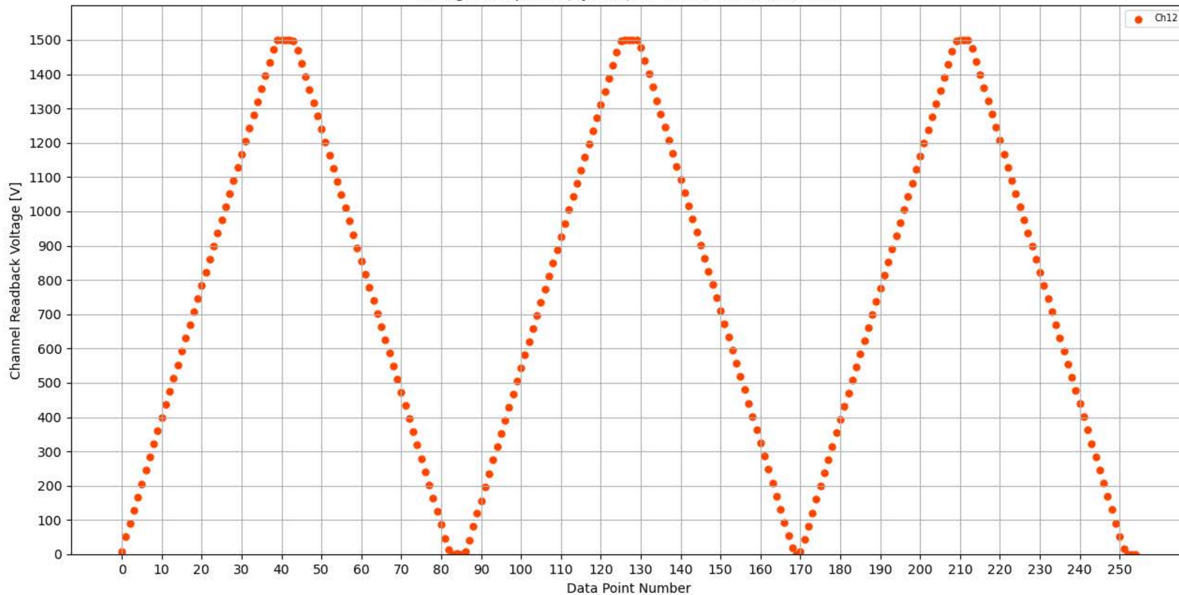
Voltage Ramp Test (Python) Bd #359, Slot #3, Ch #12
