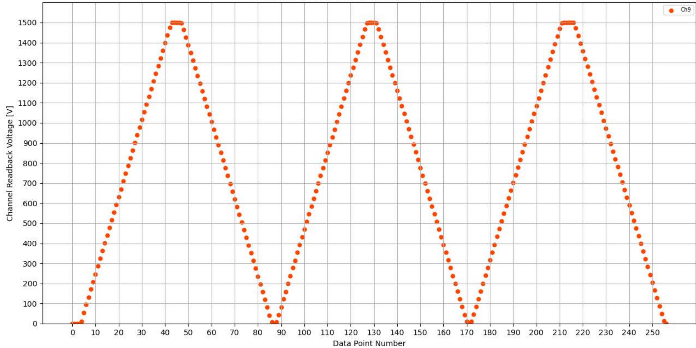
Voltage Ramp Test (Python) Bd #359, Slot #3, Ch #9
