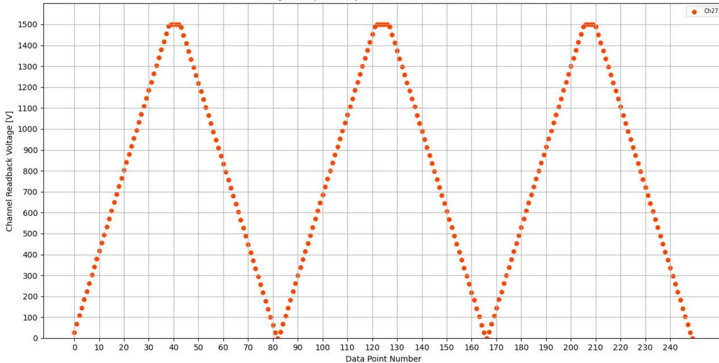
Voltage Ramp Test (Python) Bd #359, Slot #3, Ch #27
