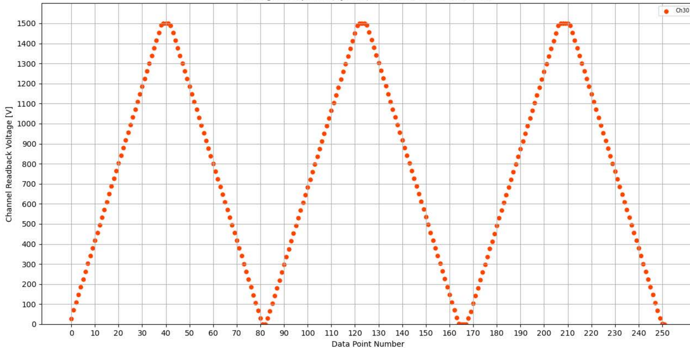
Voltage Ramp Test (Python) Bd #359, Slot #3, Ch #30
