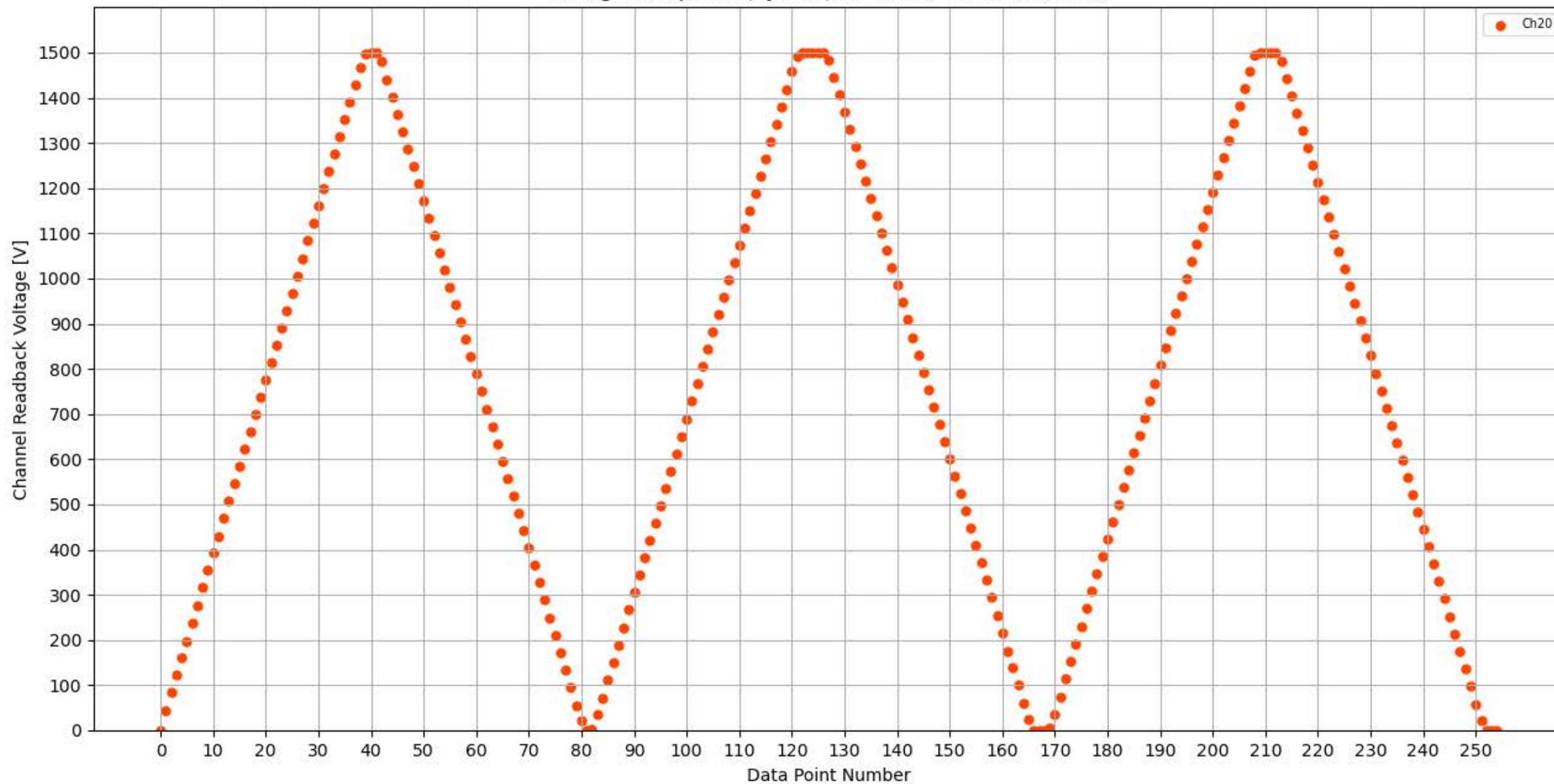
Voltage Ramp Test (Python) Bd #359, Slot #3, Ch #20
