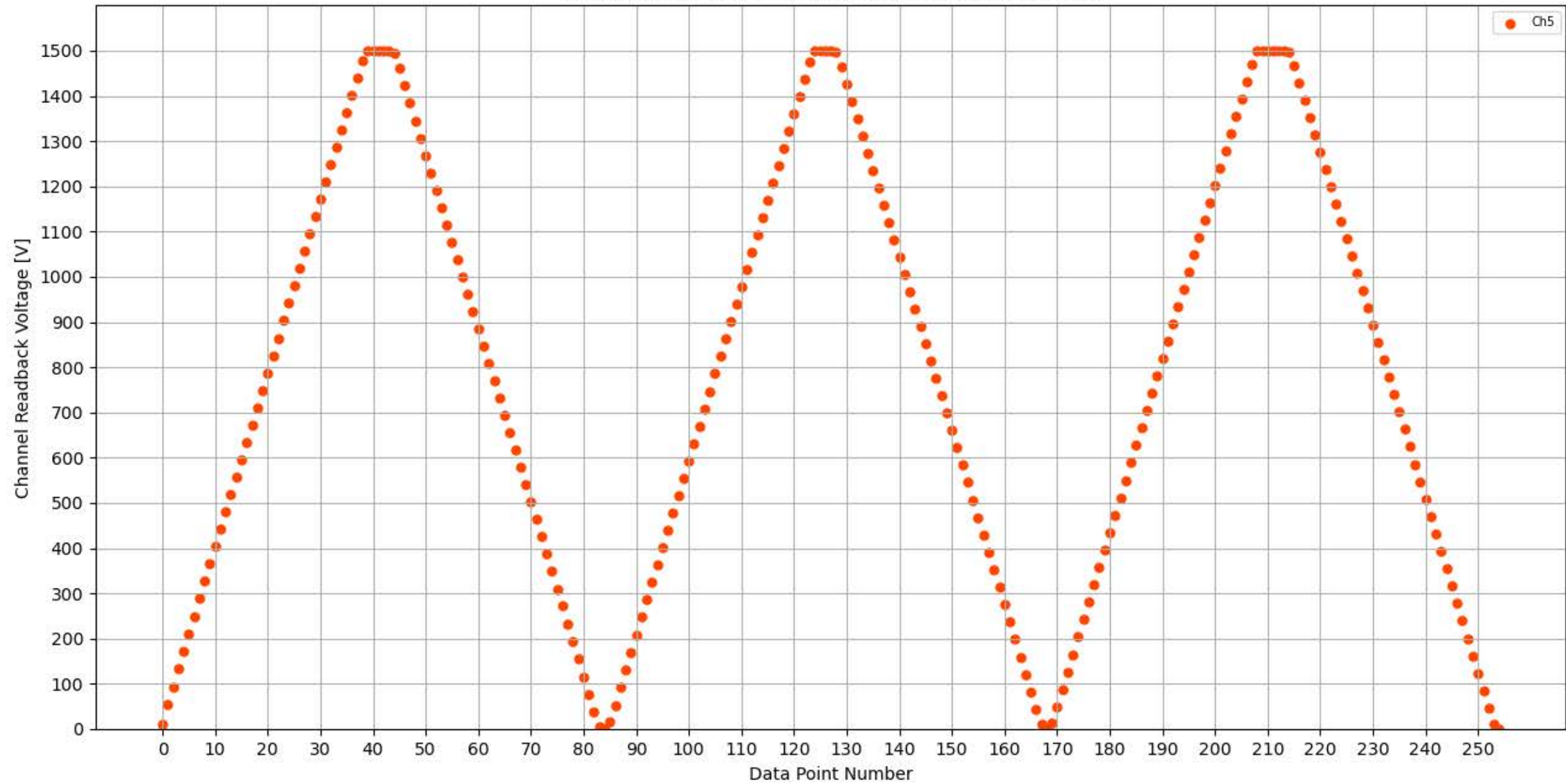
Voltage Ramp Test (Python) Bd #359, Slot #3, Ch #5
