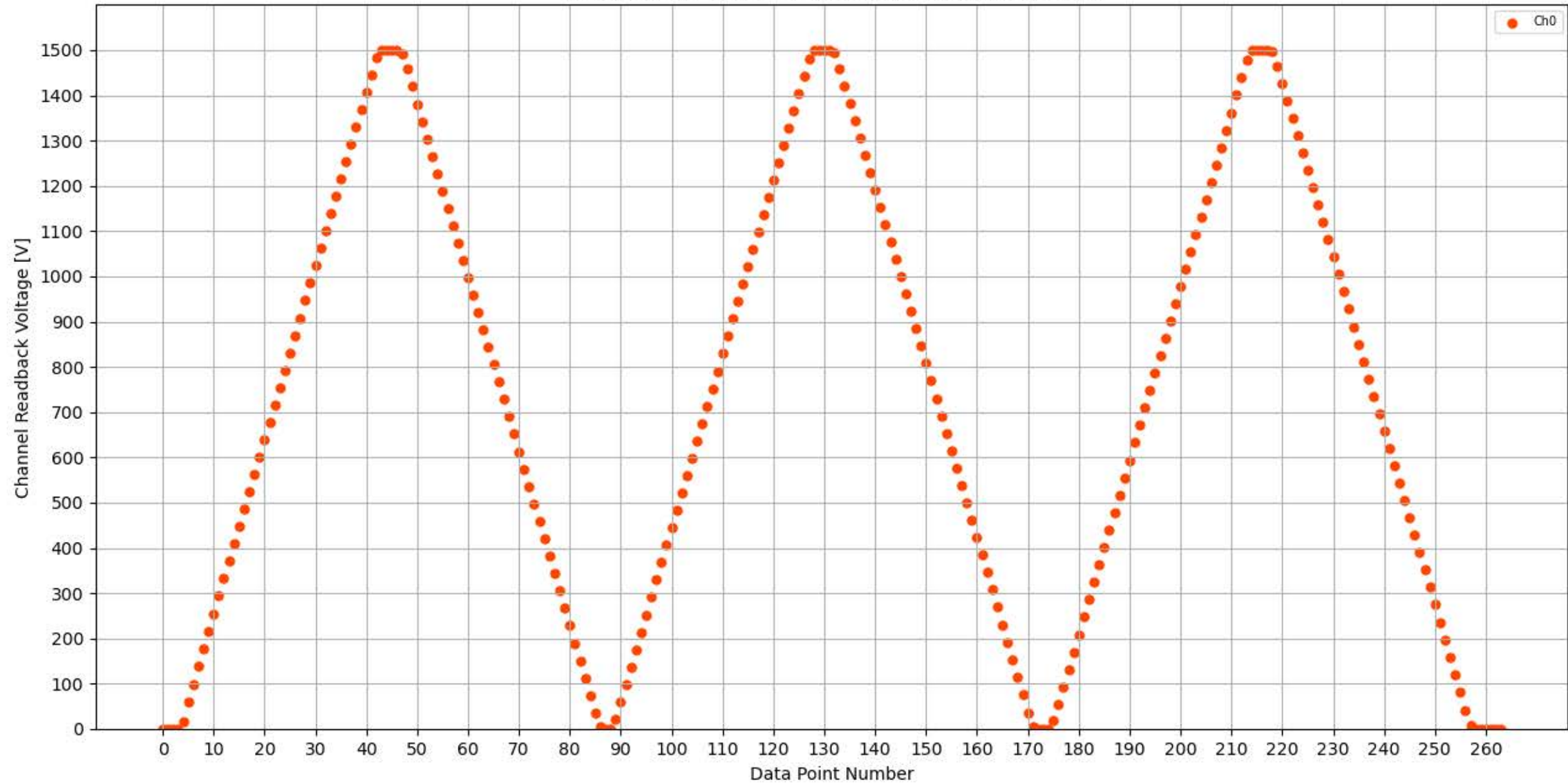
Voltage Ramp Test (Python) Bd #359, Slot #3, Ch #0
