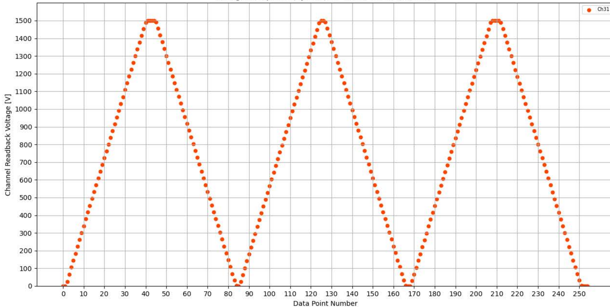
Voltage Ramp Test (Python) Bd #359, Slot #3, Ch #31
