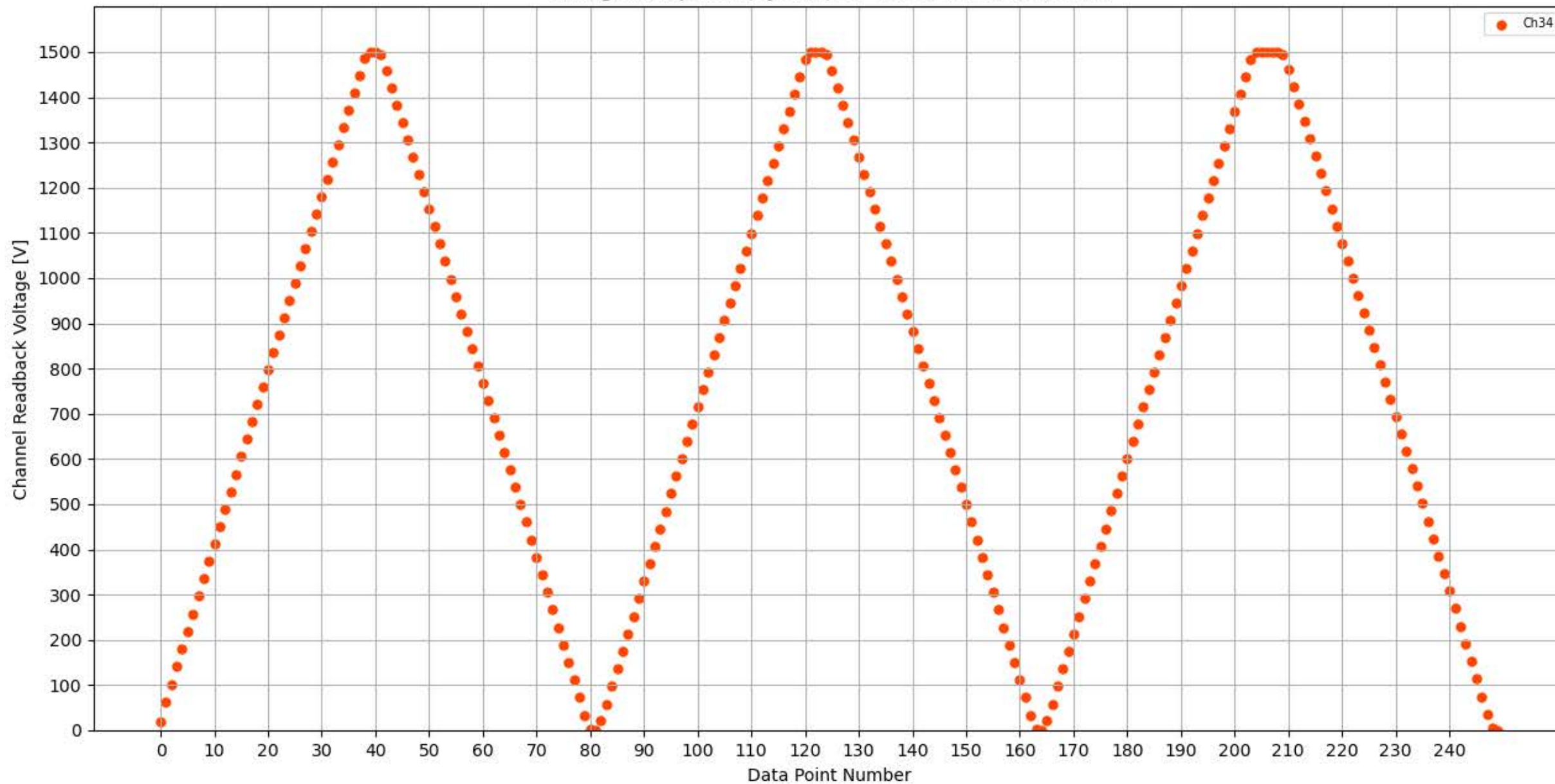
Voltage Ramp Test (Python) Bd #359, Slot #3, Ch #34
