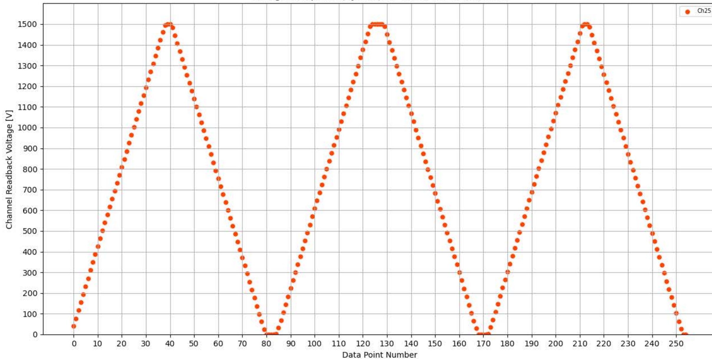
Voltage Ramp Test (Python) Bd #359, Slot #3, Ch #25
