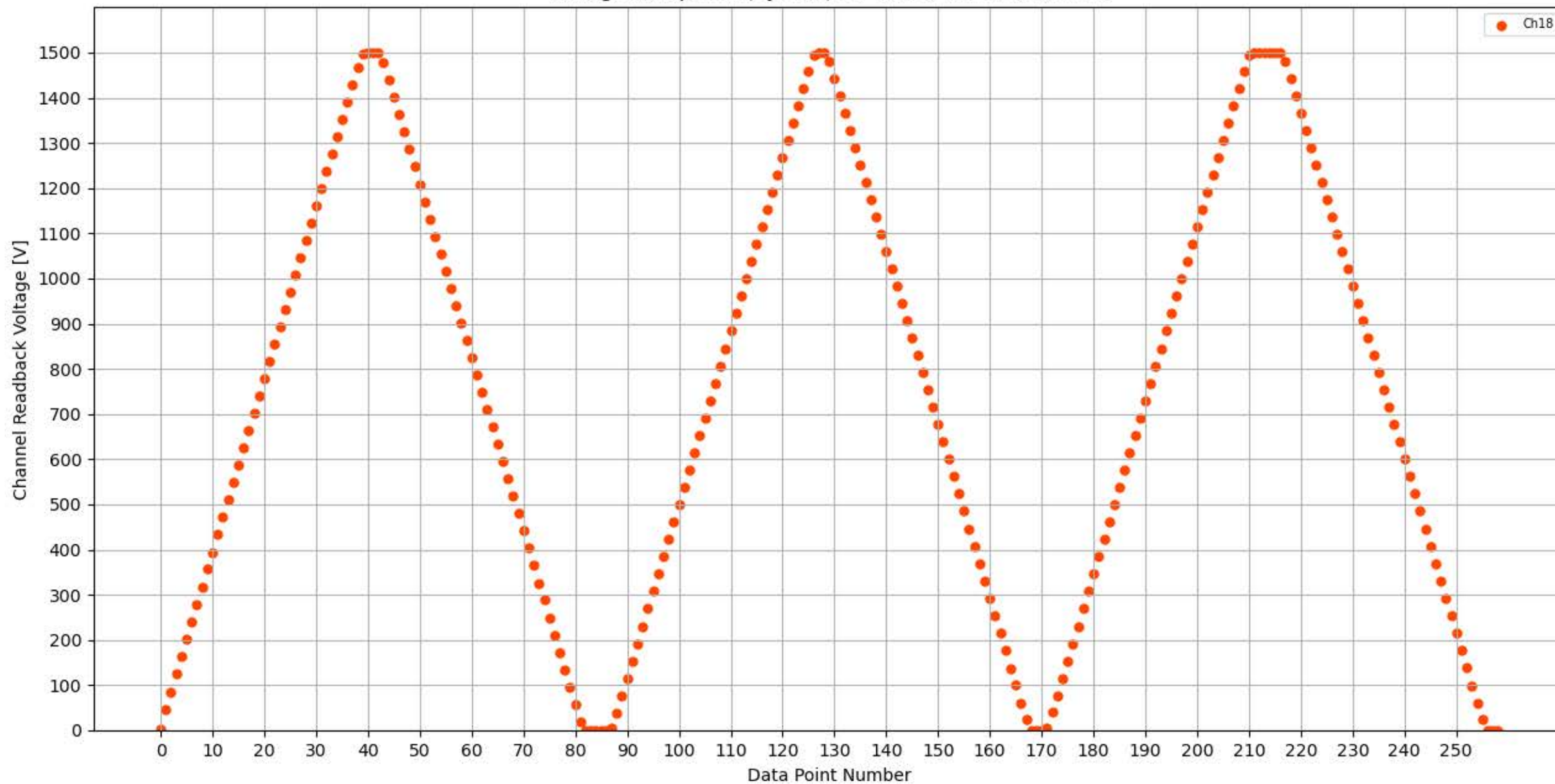
Voltage Ramp Test (Python) Bd #359, Slot #3, Ch #18
