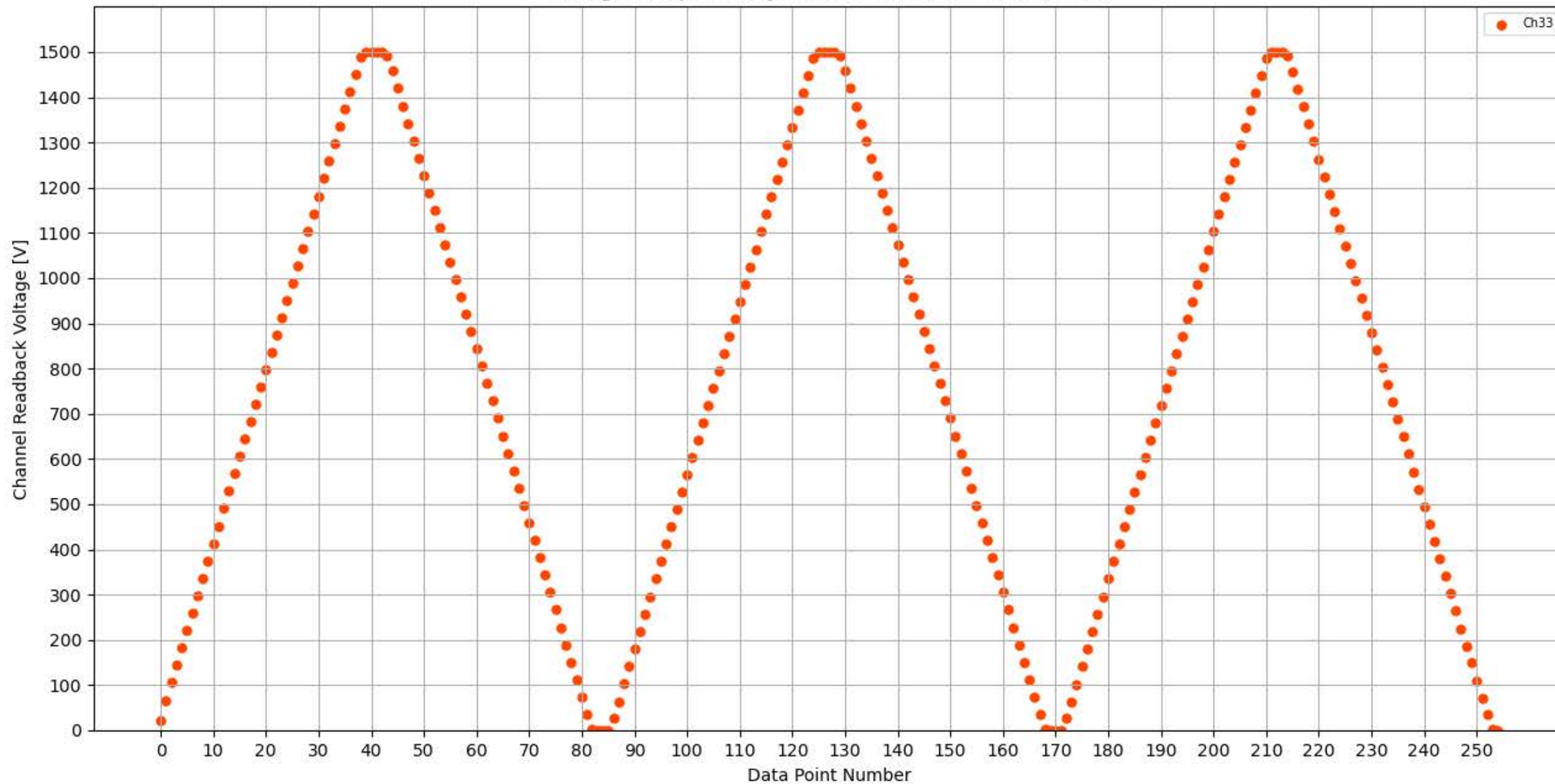
Voltage Ramp Test (Python) Bd #359, Slot #3, Ch #33
