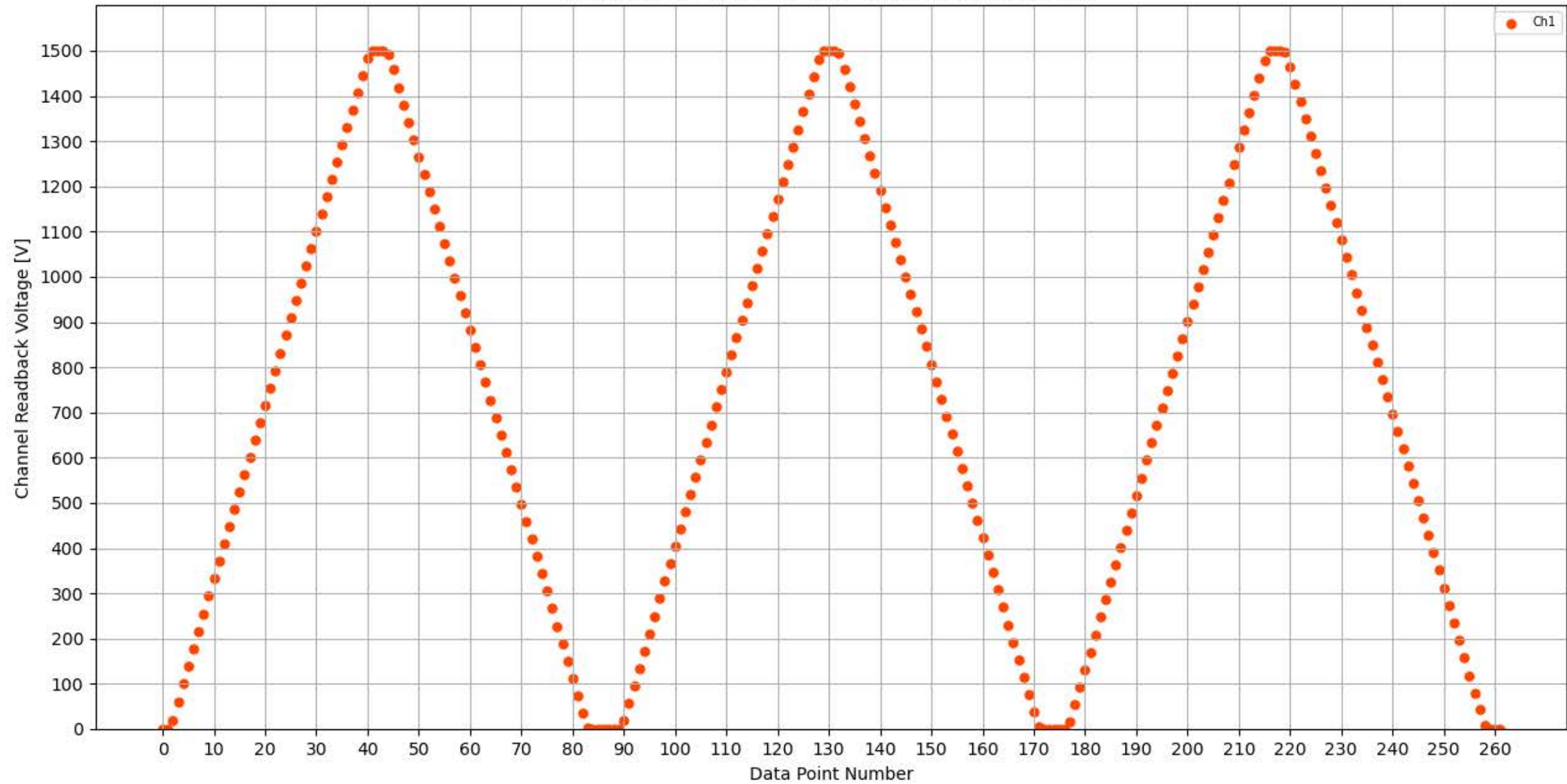
Voltage Ramp Test (Python) Bd #359, Slot #3, Ch #1
