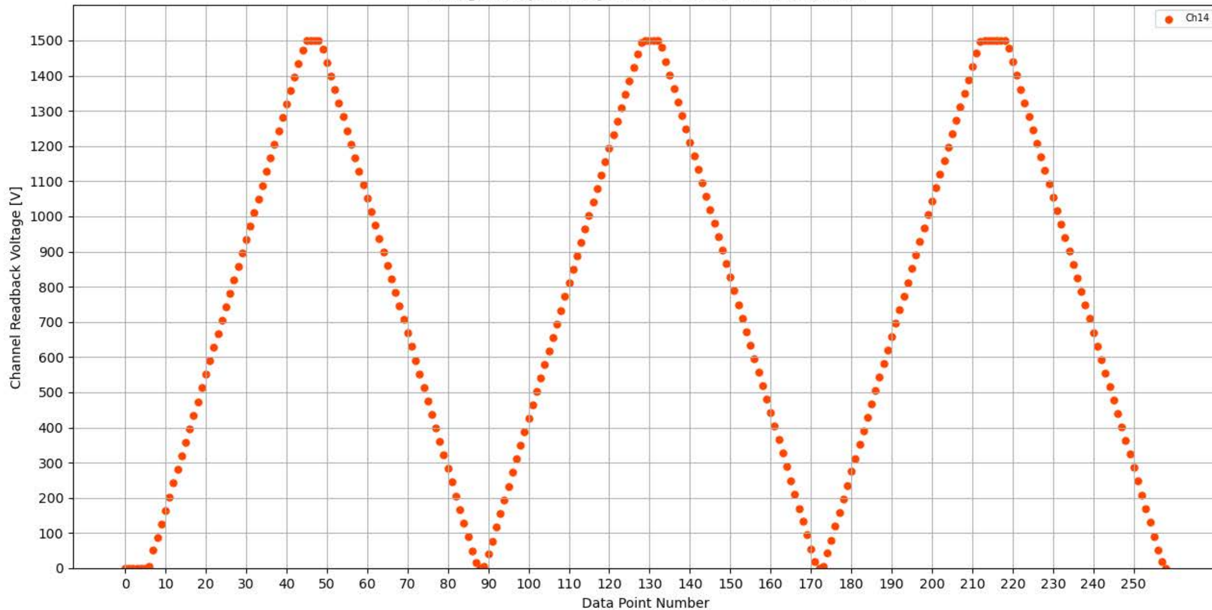
Voltage Ramp Test (Python) Bd #359, Slot #3, Ch #14
