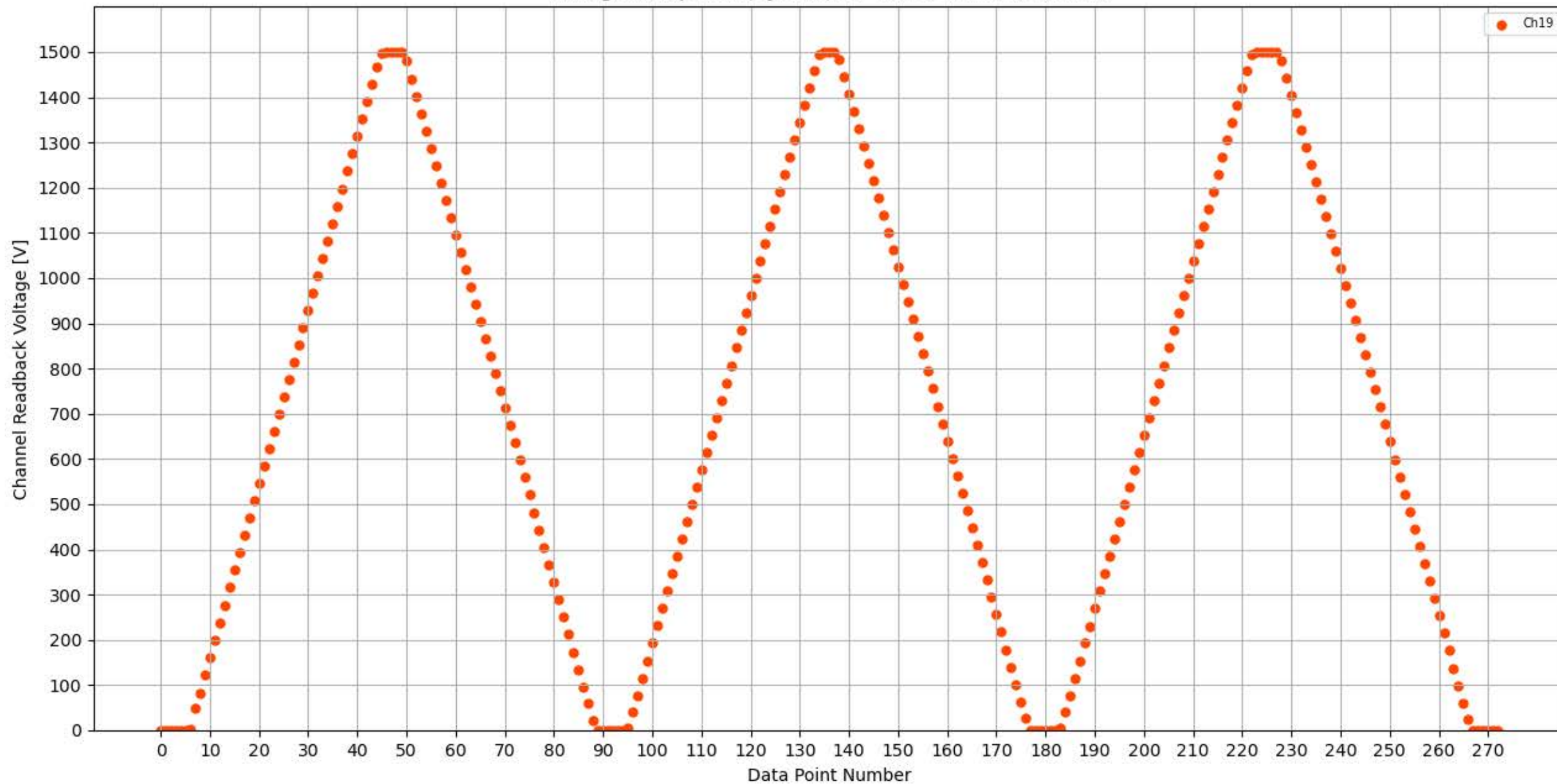
Voltage Ramp Test (Python) Bd #359, Slot #3, Ch #19
